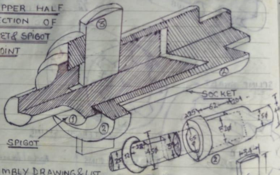
COTTER
