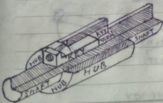
② SINGLE HEADED KEY
