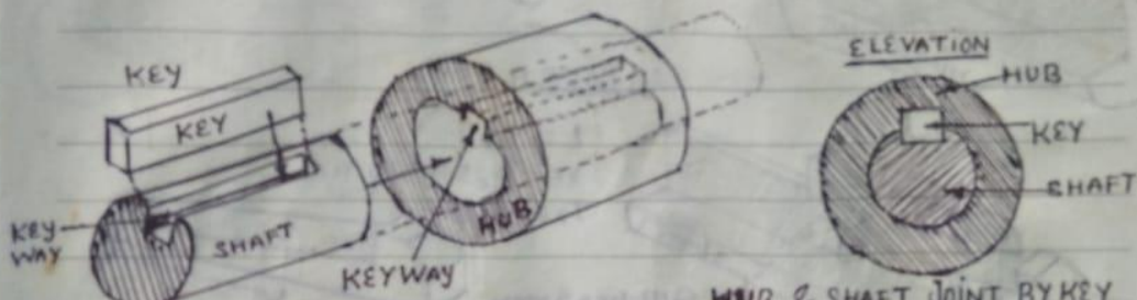
HUB & SHAFT JOINT BY KEY
